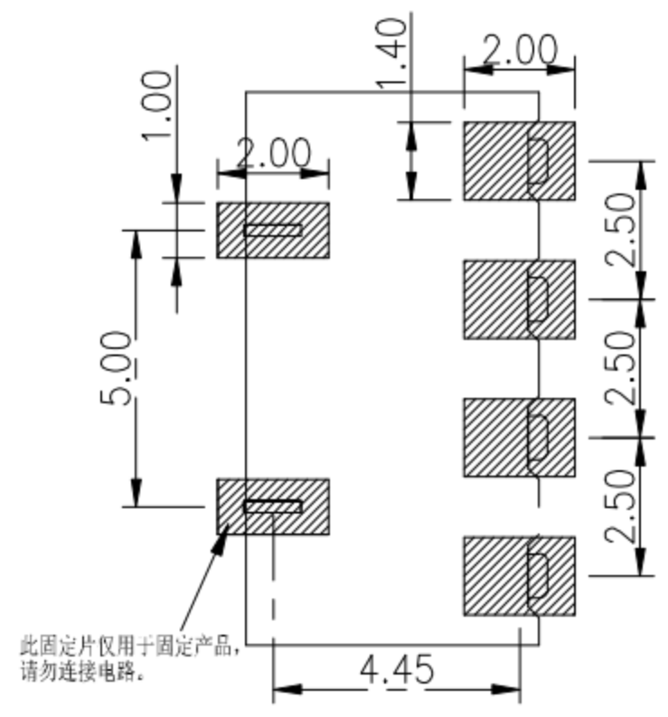
RECOMMENDED PCB LAYOUT TOP VIEW (.XX±0.05)
